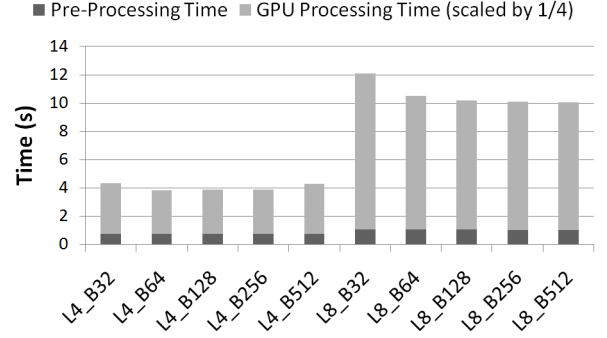
Figure 6: Total execution time filtering 32K queries over a 50MB DBLP XML document, highlighting pre-processing time on the CPU (with the common prefix optimization applied) , and GPU processing time (scaled by 1/4). The query set consists of length (L) 4 and 8 queries, while varying block sizes (B).
