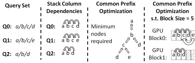
Figure 3: Sample query set shown initially, followed by the stack column dependencies for each query stack independently; these dependencies determine the propagating path of a ‘1’. A tree representation of all the queries as grouped by common prefixes is then portrayed. Finally, the query nodes are mapped to GPU blocks with a restriction on the block size.
